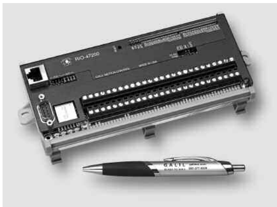
RIO-472xx provides DIN mount and screw terminals
