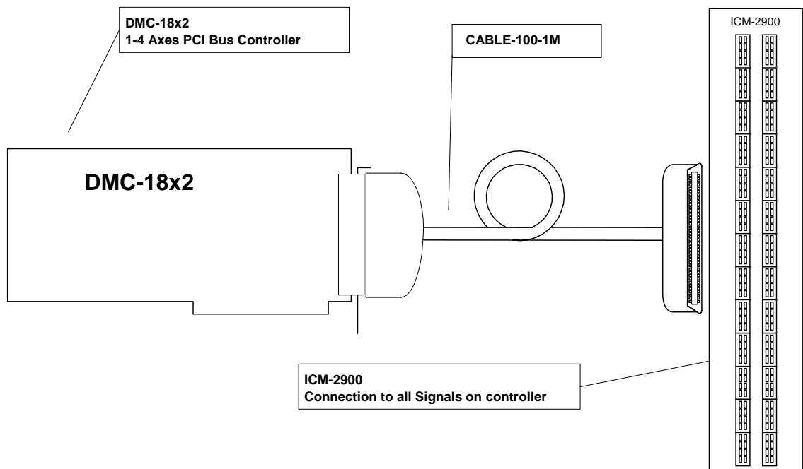
Figure 1. DMC-18x2 Controller with recommended cables for system connection.
