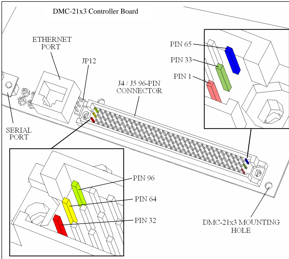
Figure 1 – DMC-21x3 J4 and J5 plug in -UP (default) configuration.
