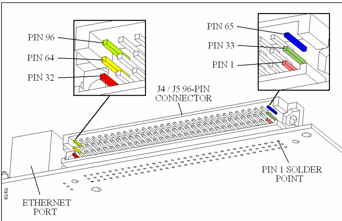
Figure 2 – DMC-21x3 J4/J5 –RA (right angle) configuration.
