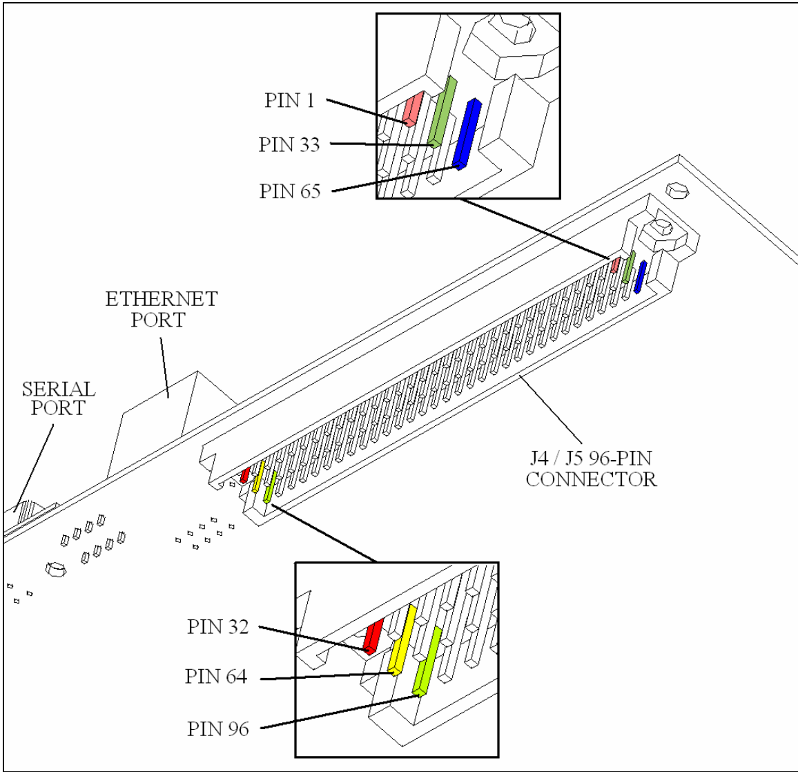
Figure 3 – DMC-21x3 J4/J5 –DOWN configuration.
