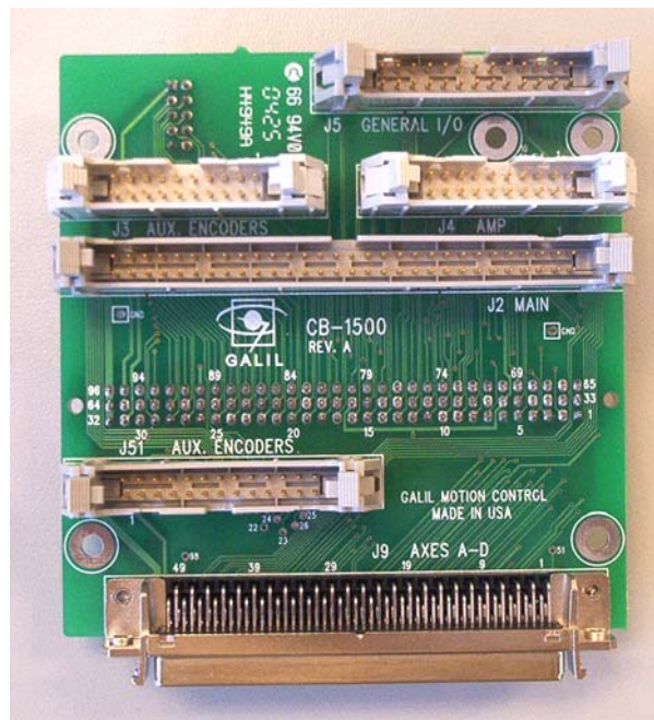
CB-1500 Interconnect Converter Board
