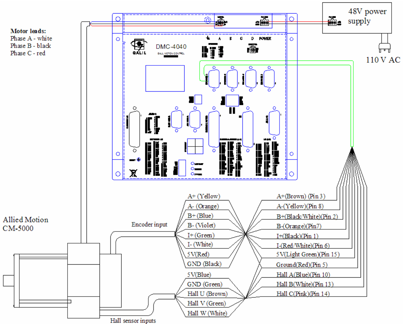
Figure 1 System Setup
