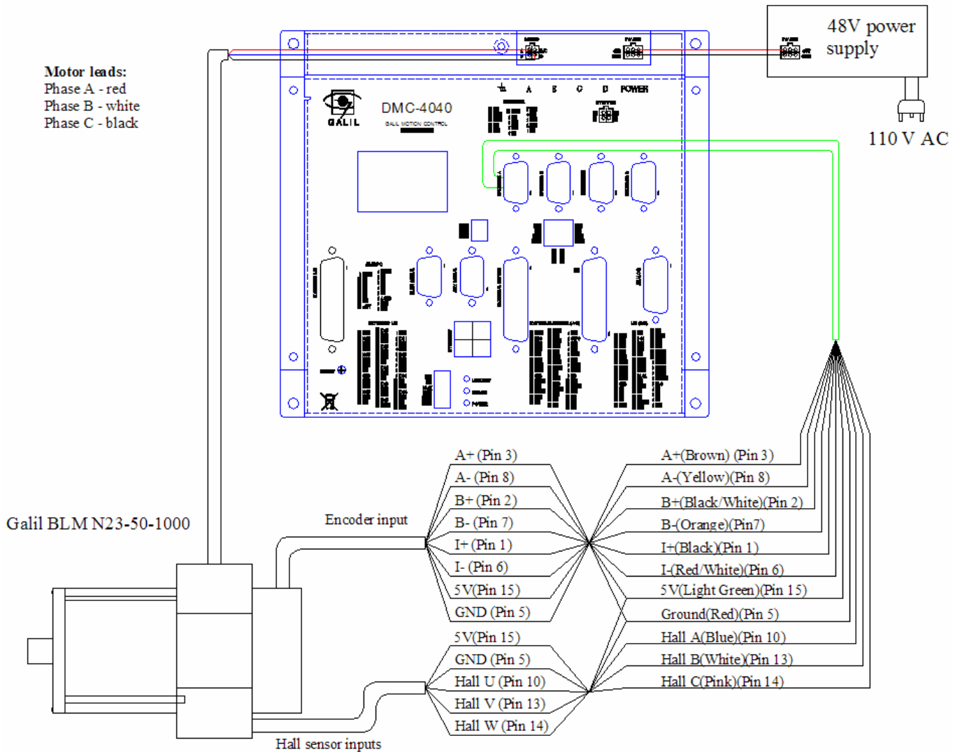
Figure 1 System setup
